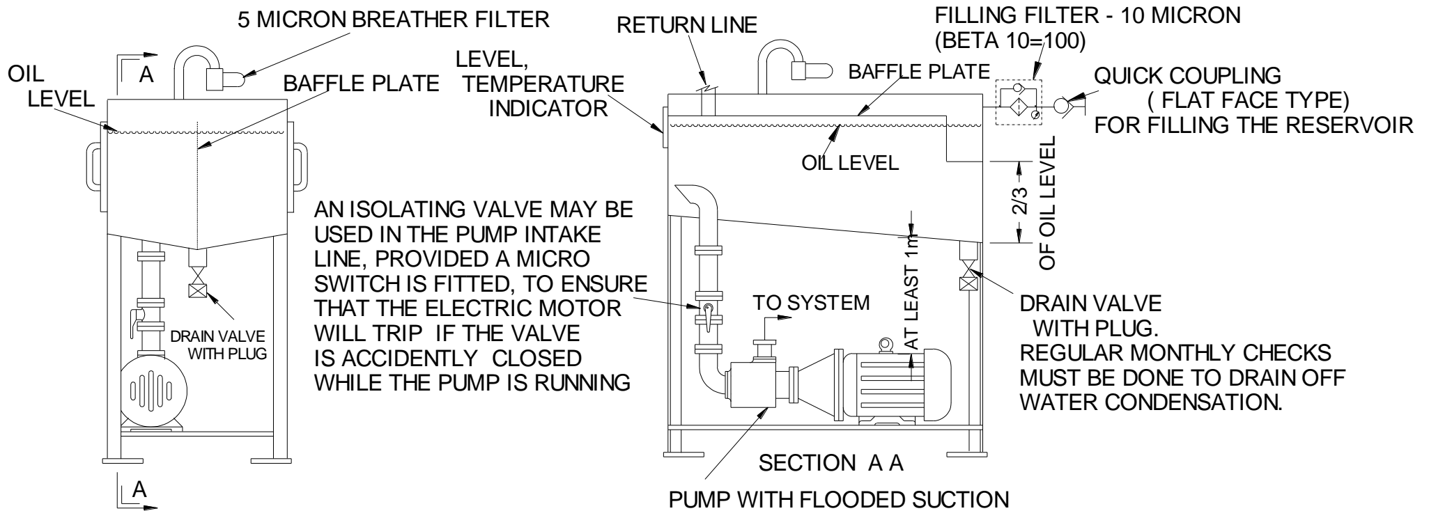
END AND SIDE VIEW OF THE RESERVOIR ASSEMBLY
